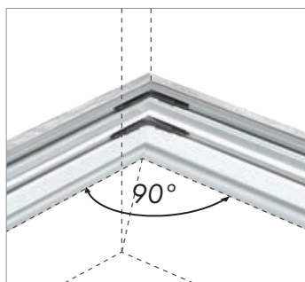
External corner
